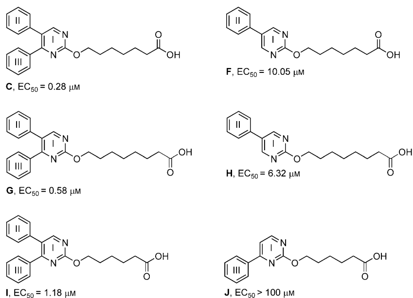
Figure 4. Structure–activity relationship for some derivatives of ligand C .
